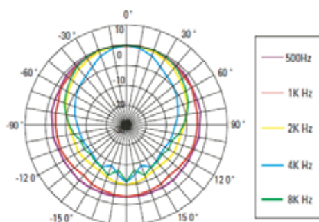
Polar Pattern
