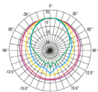
Polar Pattern
